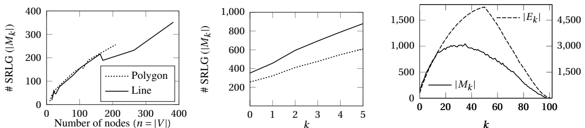
(a) The increase of the number of SRLGs with respect to the number of nodes, for k=0 . (b) The average the number of SRLGs over all networks. (c) The number of SRLGs and the number of edges in graph k -Delaunay for US Deltacom
